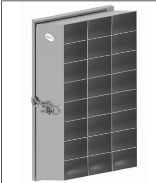
Eye Protection Holder Compartments are sized for safety glasses and may be customized for goggles and other PPE. Compartments are 3 5 / 16 " wide, 2 5 / 16 " high, and 6 1 / 2 " deep.
