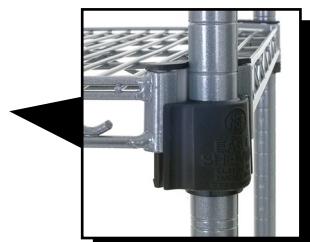
channel of shelf corner fits into slot of collar attached to split sleeve
