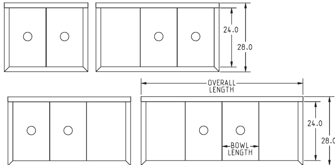
TOP VIEWS
