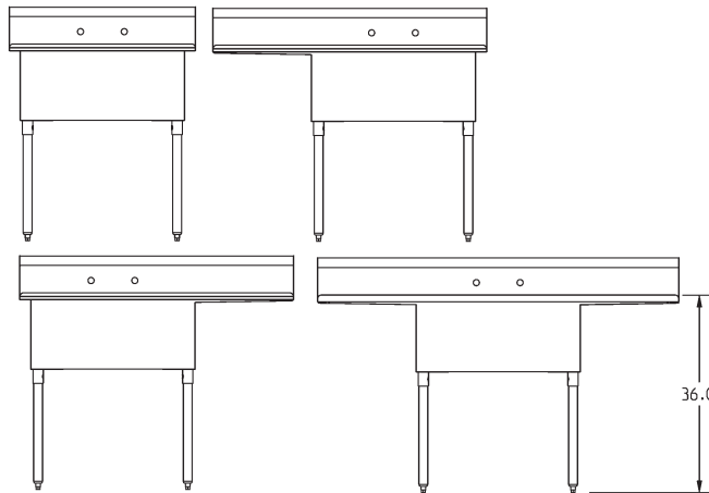
FRONT VIEWS
