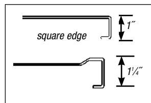
box marine edge detail 1: edges
