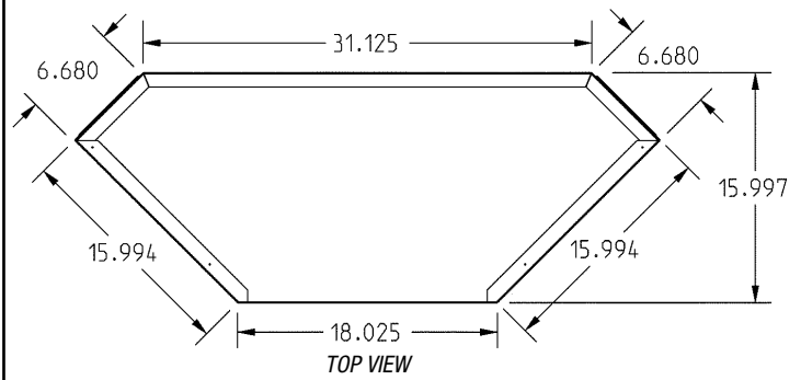
16" Cabinet Dimensions
