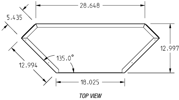
13" Cabinet Dimensions
