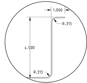
Detail #3: example of a 4 1/2" backsplash with 1" return
