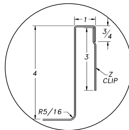
Detail #2: example of a 4" backsplash with 1" return and turn-down. Z-clip provided for wall attachment
