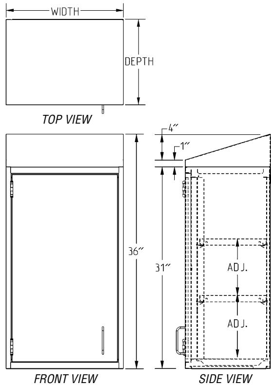
Units with Sloped Top
