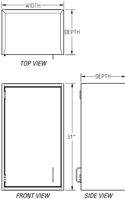
Units with Flat Top
