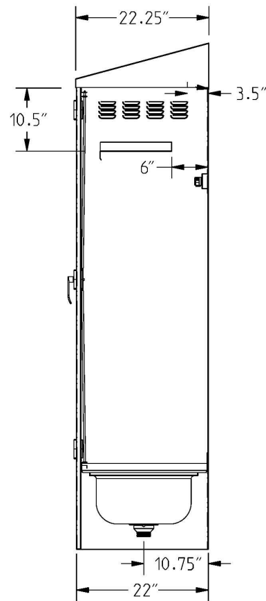
SIDE VIEW (section)
