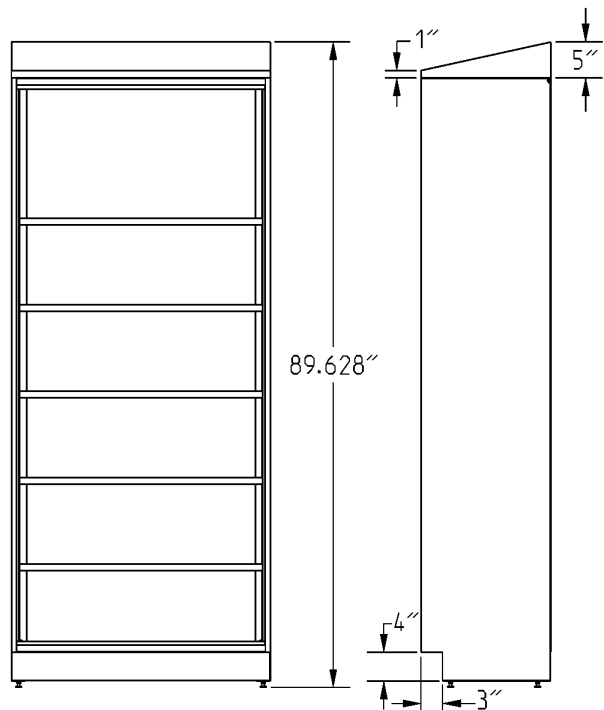
FRONT VIEW SIDE VIEW (model #SSC-TOBST-1836 shown)
