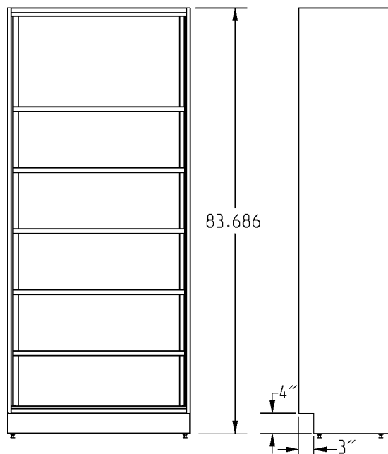
FRONT VIEW SIDE VIEW (model #SSC-TOB-1836 shown)
