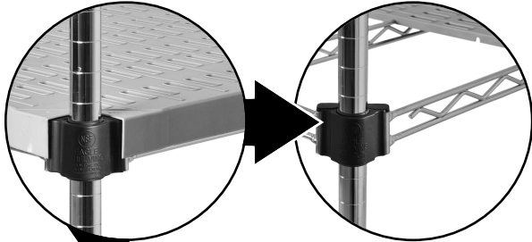
QuadPLUS® shelf mat removed, showing Quad-Adjust® wire truss frame
