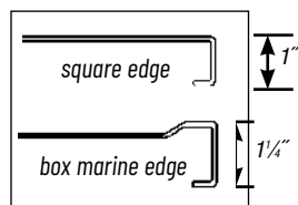
detail 1: edges
