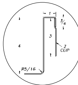
detail 2: 4" backsplash with 1" return and turndown. Z-clip provided for wall attachment.
