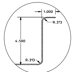
detail 3: 4-1/2" backsplash with 1" return.
