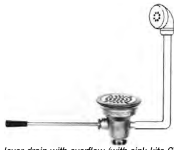
lever drain with overflow (with sink kits C)
