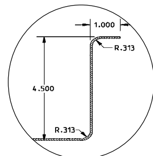
detail 3: 4-1/2" backsplash with 1" return.
