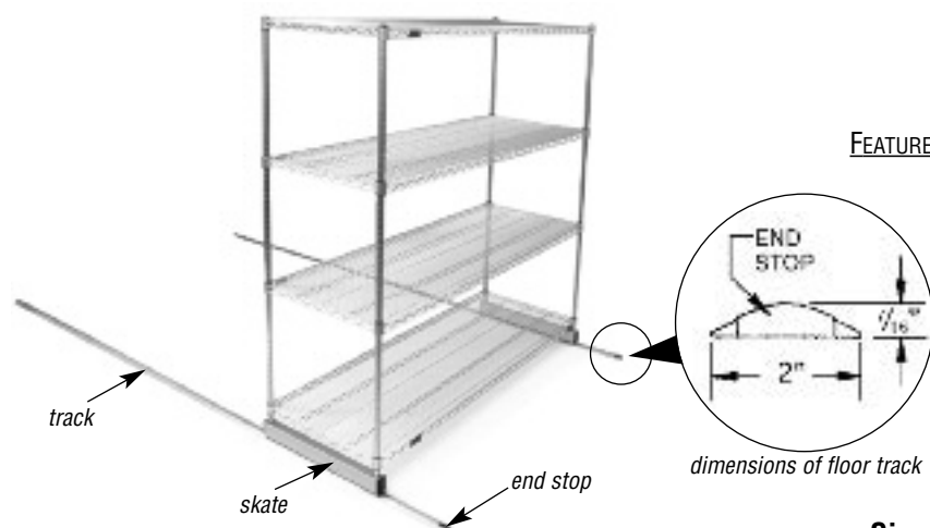
single deep unit shown assembled with wire starter unit
