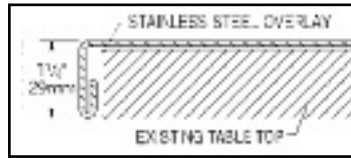
overlay fitted onto tabletop
