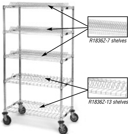
reel shelves shown in mobile unit configuration - posts and casters sold separately (see pages 8 & 9)
