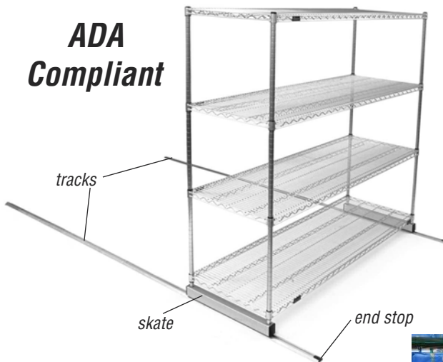
Single Deep Floor-Trak® Unit shown assembled with wire starter unit - wire shelving unit sold separately
